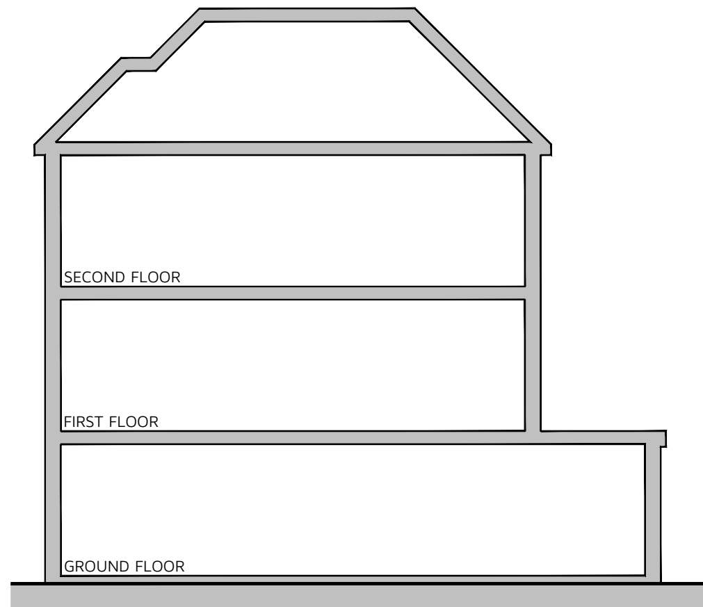
Outline Proposed Section 1:100 @ A3
