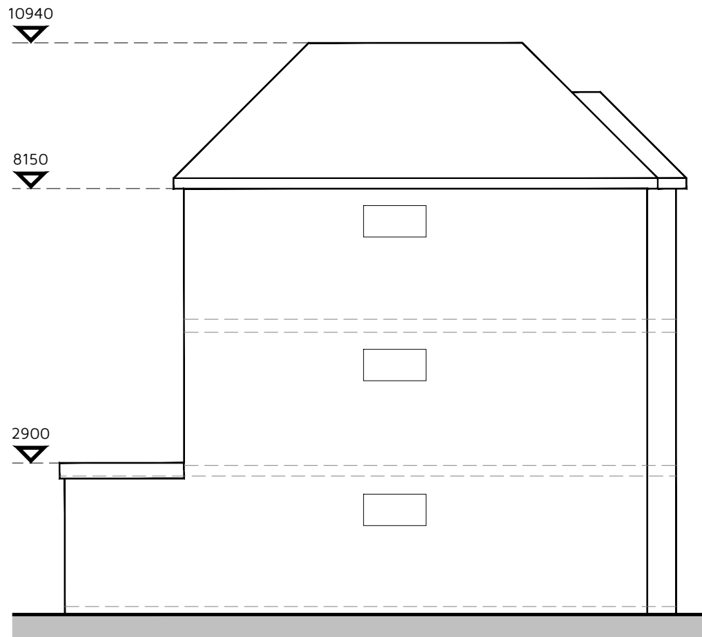
Outline Proposed Side Elevation 1:100 @ A3
