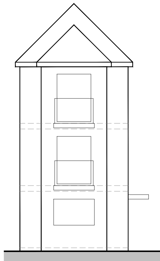
Outline Proposed Front Elevation 1:100 @ A3
